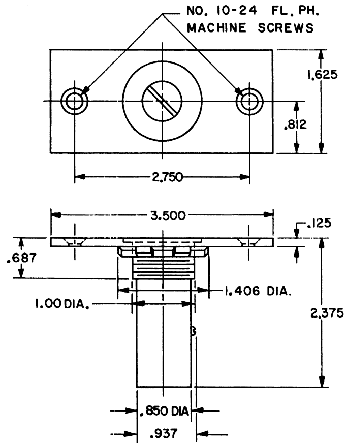
STRIKE DETAIL
