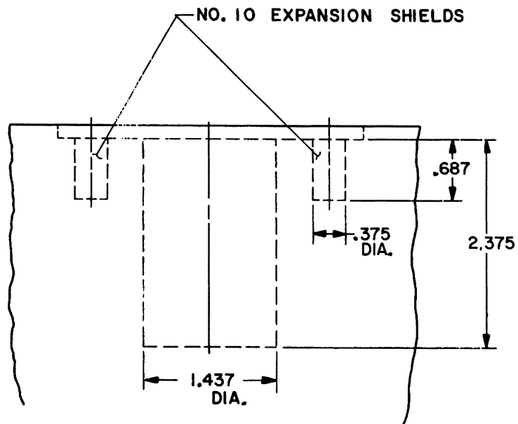
FLOOR DETAIL
