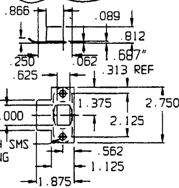
LATCH STRIKE & WROUGHT BOX DETAIL
