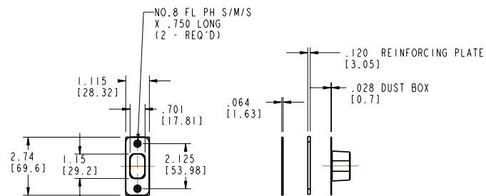
DEADBOLT STRIKE, REINFORCEMENT PLATE & DUST BOX DETAIL
