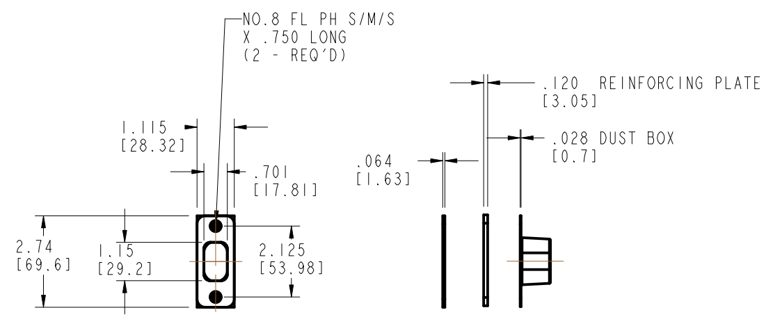
DEADBOLT STRIKE, REINFORCEMENT PLATE & DUST BOX DETAIL
