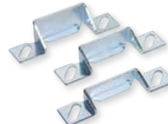
RIGID STRIKE REPLACEMENT SET FINISH: Zinc SIZE: 1/4, 3/8, 1/2" FAMILY#: Stanley: V1714 National: V1356 STOCK#: Stanley: 843268 National: 349258
