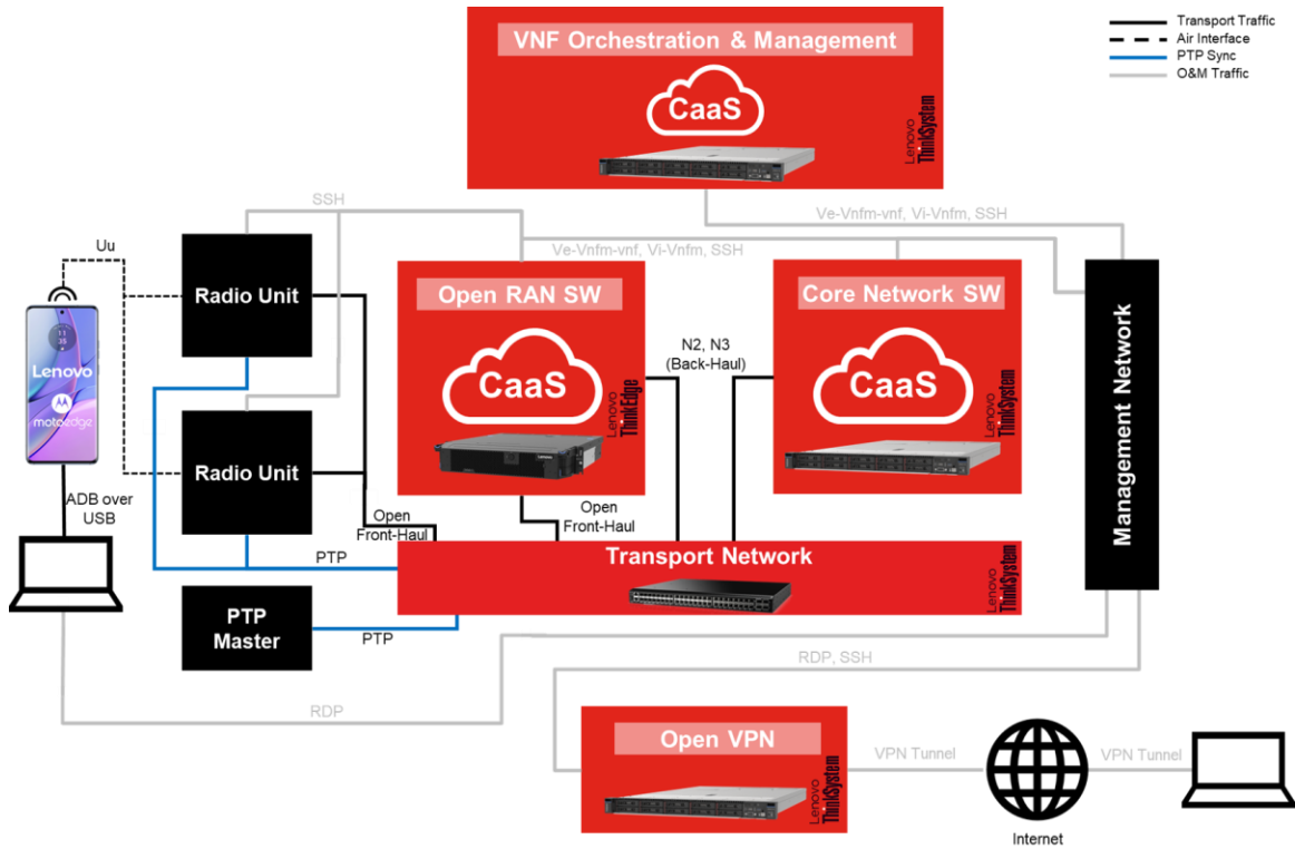
Figure 2 – Deployment and Integration Architecture
