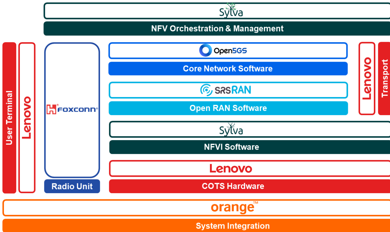
Figure 1 – Layered Deployment Blueprint
