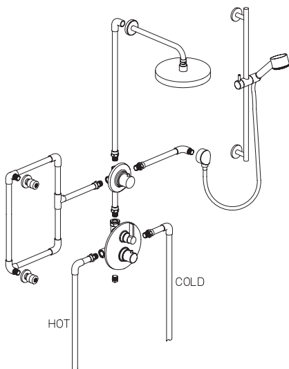
92KIT09 ½" Thermo Shower Set with Slide Bar, Shower Head and 2 Body Jets
