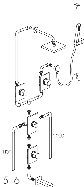
84KIT06 3/4" Thermo Shower Set with Slide Bar, Shower Head and Bath Spout
