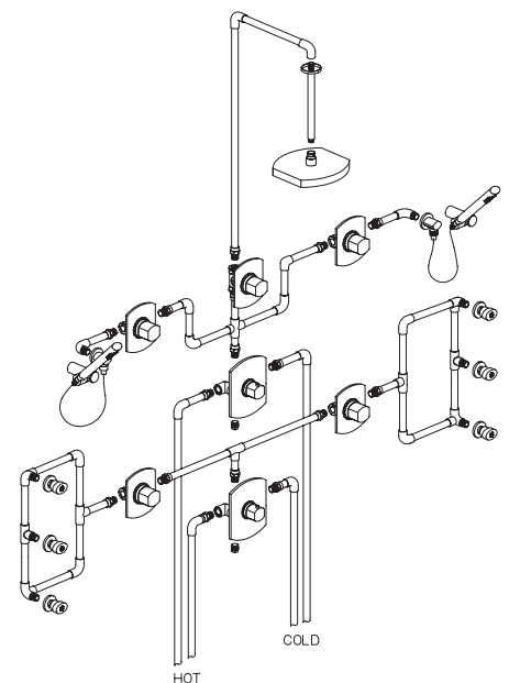
89KIT08 \frac{3}{4} " Thermo Shower Set with 2 Thermo Valve, one Ceiling Rain Shower, 2 Handshowers, and 6 Body Jets
