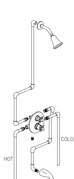
88KIT03 1/2" Thermo Valve Tub and Shower Set
