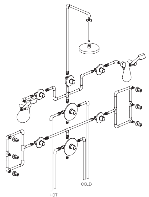
92KIT08 \frac{3}{4} " Thermo Shower Set with 2 Thermo Valve, one Ceiling Rain Shower, 2 Handshowers, and 6 Body Jets
