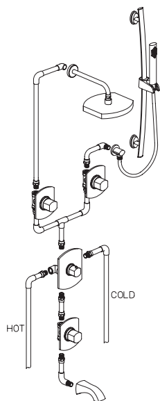
89KIT06 \frac{3}{4} " Thermo Shower Set with Slide Bar, Shower Head and Bath Spout
