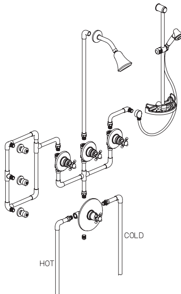
88KIT05 3/4" Thermo Shower Set with Slide Bar, Shower Head and 3 Body Jets
