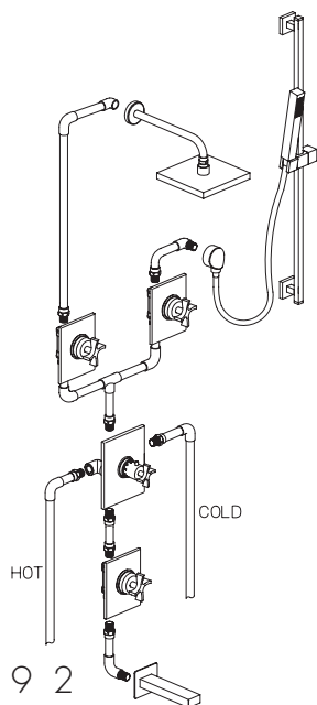
85KIT06 \frac{3}{4} " Thermo Shower Set with Slide Bar, Shower Head and Bath Spout
