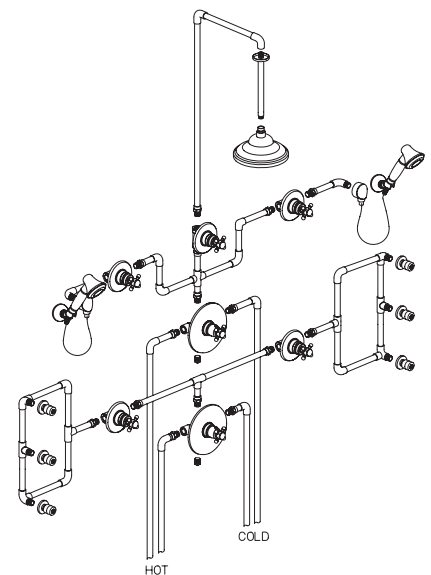
88KIT08 \frac{3}{4} " Thermo Shower Set with 2 Thermo Valve, one Ceiling Rain Shower, 2 Handshowers, and 6 Body Jets
