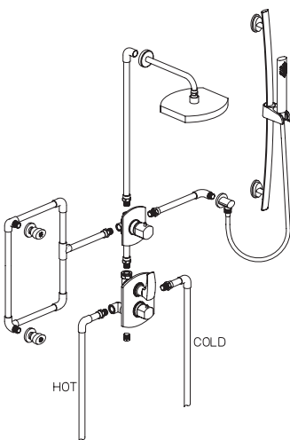
89KIT09 1/2" Thermo Shower Set with Slide Bar, Shower Head and 2 Body Jets
