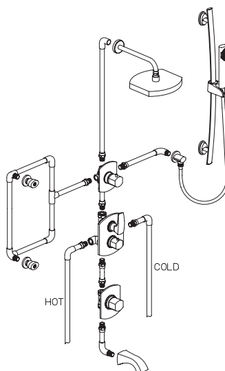
89KIT10 1/2" Thermo Shower Set with Slide Bar, Shower Head, 2 Body Jets and Bath Spout
