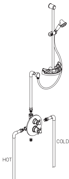
88KIT02 1/2" Thermo Shower Set with Slide Bar
