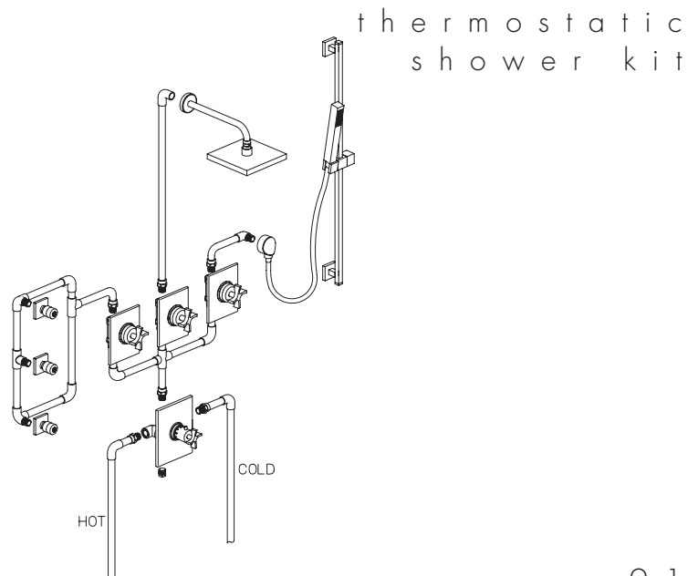
85KIT05 3/4" Thermo Shower Set with Slide Bar, Shower Head and 3 Body Jets
