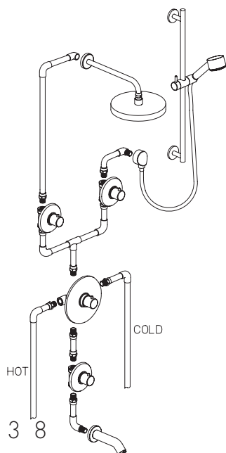
92KIT06 \frac{3}{4} " Thermo Shower Set with Slide Bar, Shower Head and Bath Spout
