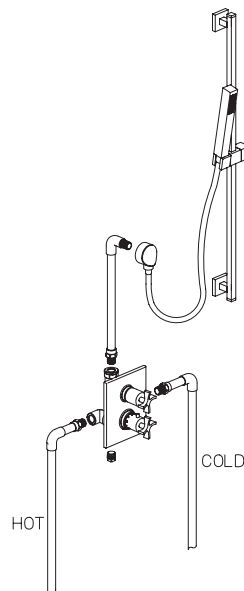
85KIT02 1/2" Thermo Shower Set with Slide Bar
