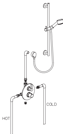
92KIT02 1/2" Thermo Shower Set with Slide Bar
