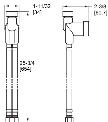
Mixing Valve
