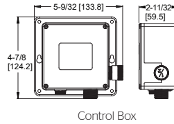
Control Box
