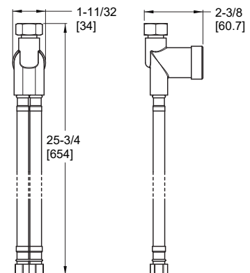
Mixing Valve
