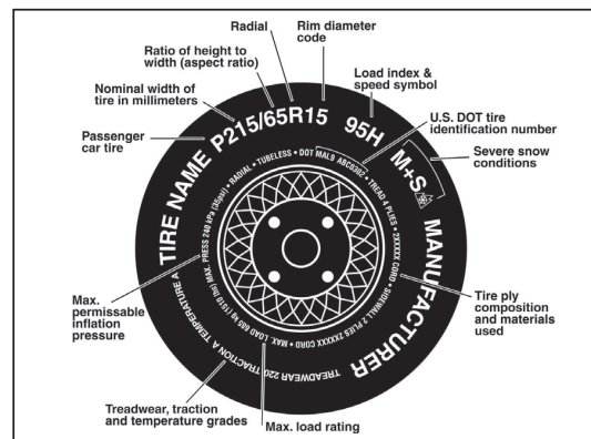
Figure 3: Typical Passenger Tire Markings
